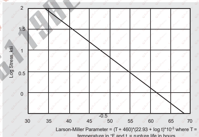
Figure 7. Creep-rupture strength of INCOLOY alloy 800HT (UNS N08811)
